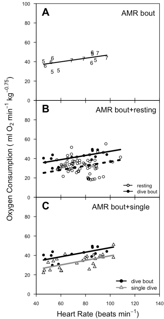
Figure A3. 6 The relationship between average heart rate ( f_h ) and average metabolic rate ( \dot{V}_{O_2} = AMR) for Steller sea lions averaged over a dive bout cycle (dives+surface intervals, A) was different than when animals were resting in water (B) and also different than the relationship over a single dive cycle (C). See Table 3.1 for Animal ID to corresponding animal number.
