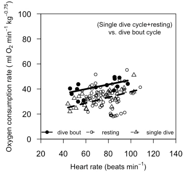
Figure 3. 4 The relationship between heart rate ( fh ) and oxygen consumption rate ( \dot{V}_{O_2} ) when Steller sea lions were resting (RMR, open circles) did not differ from that for predicting average metabolic rate over a single dive cycle (AMR, open triangles), but did differ from the relationship for predicting AMR over a dive bout cycle (closed circles). Equations were derived using mixed-effects linear models with a repeated measures framework.
