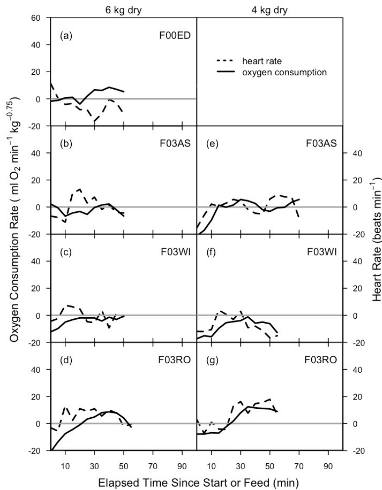
Fig. 2.5 Relative heart rate ( fh , dashed line) and oxygen consumption ( \dot{V}_{O_2} , solid line) of Steller sea lions above baseline (fed 0 kg) values (grey line at zero) following a single meal of 4 or 6 kg (dry 4kg and dry 6kg trials). All animals were dry and remained in a metabolic chamber during the trials. Note that F00ED did not complete a dry 4kg trial. Regressions were derived using mixed-effects linear models within a repeated measures framework (see Fig. A2.8 for corresponding trials in water).
