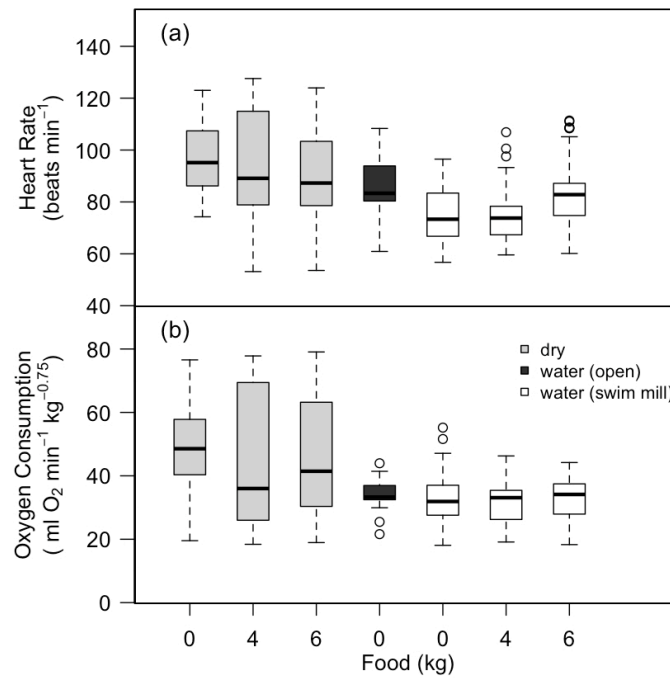
Figure A2. 1 Box-and-whiskers plot of heart rate ( fh ) and oxygen consumption ( \dot{V}_{O_2} ) showing minimum, median, and maximum fh (a) and \dot{V}_{O_2} (b) for dry (metabolic chamber), water (open), and water (swim mill) trials by amount of food digested (kg).
