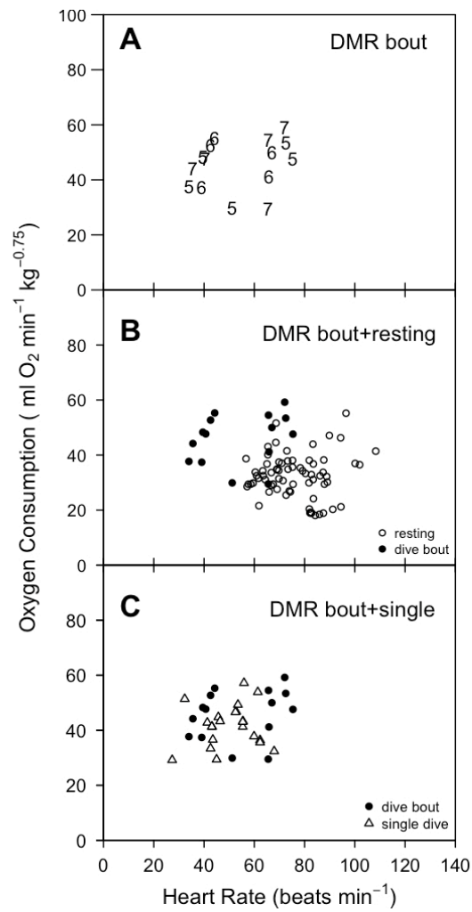
Figure A3. 4 The relationship between diving heart rate ( f_h ) and diving metabolic rate ( \dot{V}_{O_2} =DMR) for Steller sea lions over a dive bout (A) was not significantly linear. Combining DMR for dive bouts with data collected when animals were resting (B) or with data collected when animals were executing a single dive (C) also yielded non-linear results. See Table 3.1 for Animal ID to corresponding animal number.
