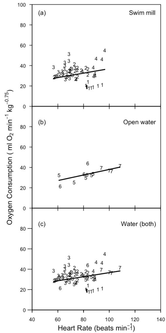
Figure A2. 2 The relationship between heart rate ( f_h ) and oxygen consumption ( \dot{V}_{O_2} ) fasted in a swim mill (a) and resting at the surface in open water (b) were not different. Therefore both trial types were combined and used as the baseline (c) for feeding (Chapter 2) and diving (Chapter 3) trials (water comp in Chapter 2 equivalent to RMR in Chapter 3).
