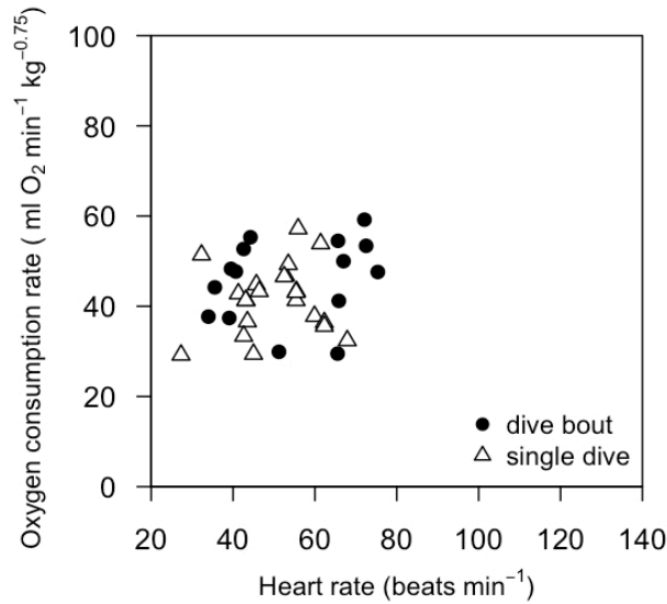
Figure 3. 2 The relationships between diving heart rate ( fh ) and diving metabolic rate (DMR) for Steller sea lions over a dive bout (closed circles) or over a single dive (open triangles) were not significantly linear.
