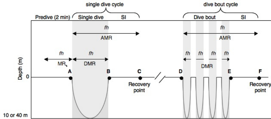
Figure 3. 1 Schematic diagram of a Steller sea lion dive trial showing dive depth (0-40 m) on the y-axis and time on the x-axis. The figure illustrates the varying intervals of average heart rate ( fh ) and oxygen consumption ( \dot{V}_{O_2} ) used to calculate different predictive equations over dives (highlighted in grey) and surface intervals (in white at 0 m depth). Standard metabolic rate or pre-dive ( MR_s ) was an average over 2 min prior to the initial dive. Average metabolic rate (AMR) for a single dive or dive bout used fh and \dot{V}_{O_2} data from the start of the dive up until the post-dive recovery point (C, set at \pm 2\% of MR_s ), which were averaged across the total dive cycle duration (dive time plus surface interval, SI). Diving metabolic rate (DMR) over a single dive or dive bout included fh data during the underwater portions only, and \dot{V}_{O_2} data only in excess of MR_s (see Fig. 3.2), averaged across total dive duration.
