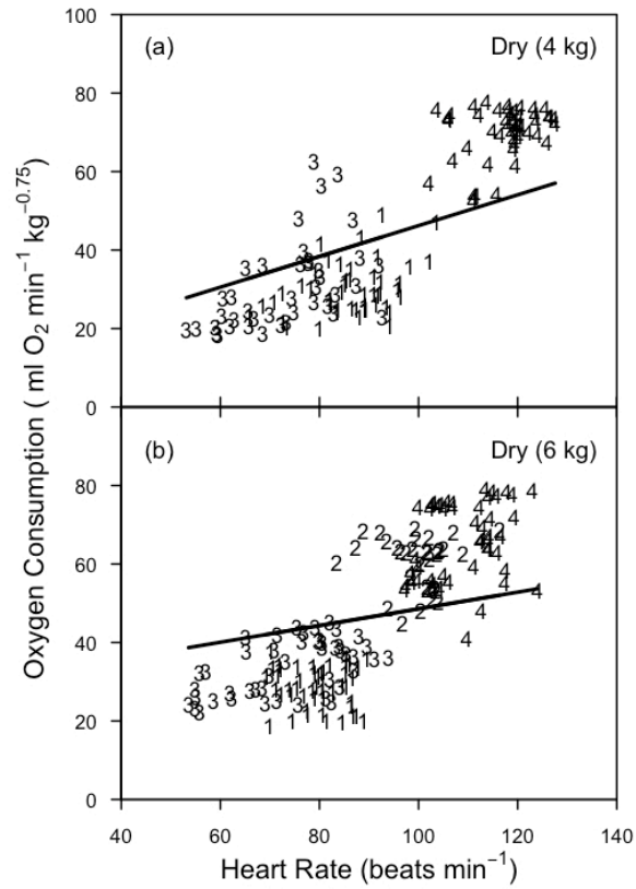
Figure A2. 3 Feeding sea lions a meal of 4 or 6 kg on land did not significantly change the relationship between heart rate and oxygen consumption. Therefore a single equation was used to predict \dot{V}_{O_2} of animals that were fasted or fed on land.
