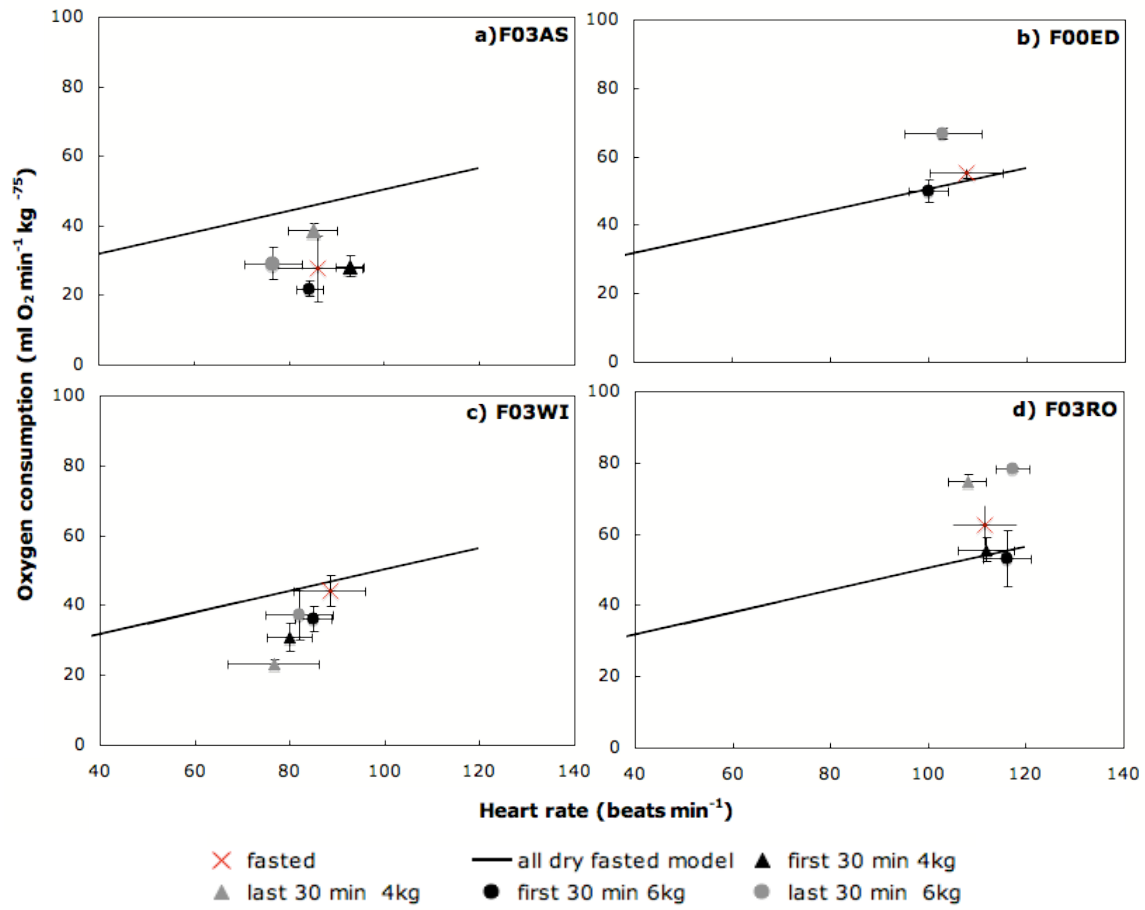
Figure A2. 4 Comparison of average fh and \dot{V}_{O_2} for dry trials. Average fh and \dot{V}_{O_2} over entire dry fasted trial (X), average fh and over first 30 minutes (black triangle) and last 30 minutes of dry 4kg (grey triangle), and average fh and over first 30 minutes (black circle) and last 30 minutes of dry 6kg (grey circle). Results showed that feeding does not uniformly move points along the “fasted” line.
