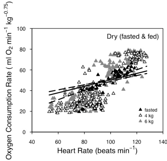
Figure 2. 3 The relationship between heart rate ( fh ) and oxygen consumption ( \dot{V}_{O_2} ) did not differ among Steller sea lions that were fasting (black triangles), or feeding 4 kg (open triangles) and 6 kg (grey triangles). A single equation (solid line) derived using mixed-effects linear models within a repeated measures' framework was therefore used to predict \dot{V}_{O_2} on land. The 95% bootstrap confidence intervals are indicated with dashed lines.
