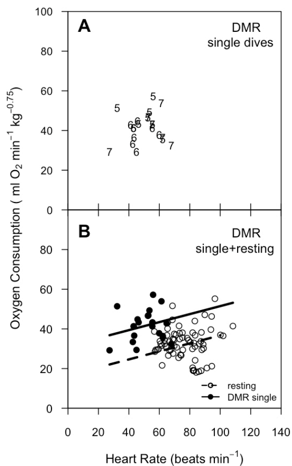
Figure A3.3 The relationship between heart rate ( fh ) and diving metabolic rate ( \dot{V}_{O_2} = DMR) averaged over a single dive (dive only) was not significantly linear (A). However, when combined with resting, the fh :DMR relationship for single dives was different than when animals were resting (RMR) in water (B). See Table 3.1 for Animal ID to corresponding animal number.
