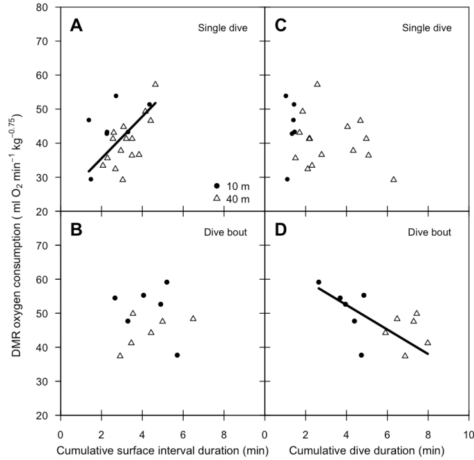
Figure 3.3 The relationship between dive characteristics and diving metabolic rate (DMR) for single dives and dive bouts. DMR increased with surface recovery time for single dives (A), but not for dive bouts (B). DMR decreased as cumulative dive duration increased for dive bouts (D), but not for single dives (C). Dive depth (10 m = closed circles, 40 m = open triangles) did not alter any of the relationships. For bout dives, all durations are cumulative, with the surface interval also incorporating the period until oxygen consumption recovered to within 2% of MR_s . Equations were derived using mixed-effects linear models with a repeated measures framework.
