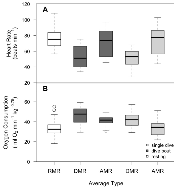
Figure A3. 2 Box-and-whiskers plot showing minimum, median, and maximum heart rate ( fh ) and oxygen consumption \dot{V}_{O_2} for animals resting in water (white), averaged over dive bouts (dark grey), or averaged over single dives (light grey). Water composite includes data when animals were resting in a swim mill and resting at the surface of open water. Diving metabolic rate (DMR) includes data averaged over single dives or several dives in dive bout. Average metabolic rate (AMR) includes data averaged over a complete dive cycle (dive +surface interval) or entire dive bout (multiple dives and surface intervals).
