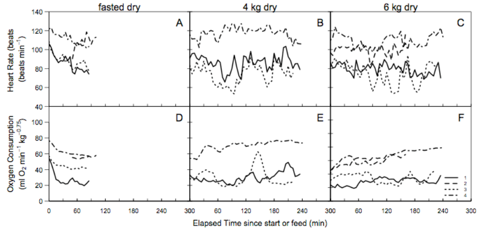
Figure A2. 6 Heart rate ( fh ) and oxygen consumption ( \dot{V}_{O_2} ) changes as a function of time for dry fasted (a, d), dry 4kg (b, e) and dry 6kg (c, f) in animals 1-4. See Table 2.1 for Animal ID to corresponding animal number.
