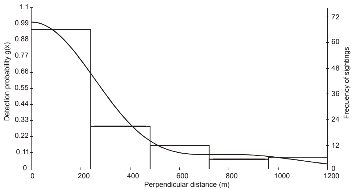
Figure 8. Probability detection distribution for perpendicular sighting distances of Dall's porpoise. Bars represent the frequency of sightings and the line represents the half-normal/cosine model of best fit, truncated at 1,200 m.
