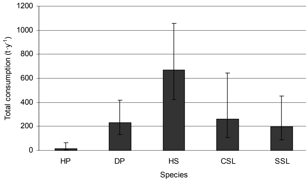
Figure 43. Estimated total consumption ( t \cdot y^{-1} ) by marine mammal species in the Strait of Georgia study area. DP = Dall's porpoise, HP = harbour porpoise, HS = harbour seals, CSL = California sea lions, SSL = Steller sea lions. Ranges are calculated based on the 95% confidence intervals obtained from DISTANCE abundance estimates.
