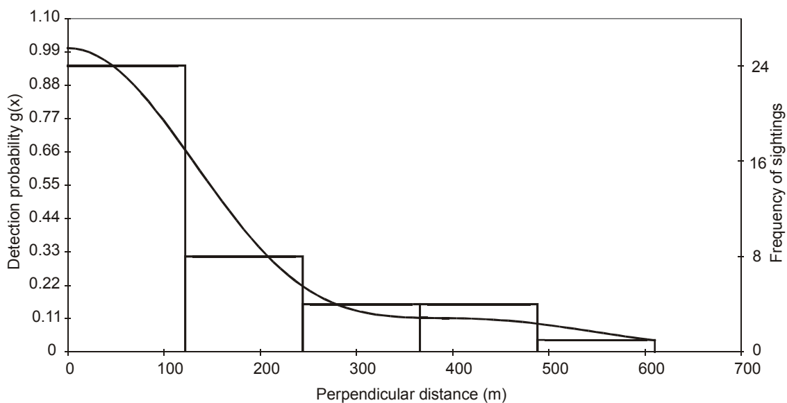
Figure 27. Probability detection distribution for perpendicular sighting distances of California sea lions. Bars represent the frequency of sightings and the line represents the negative-exponential/simple model of best fit, truncated at 610 m.
