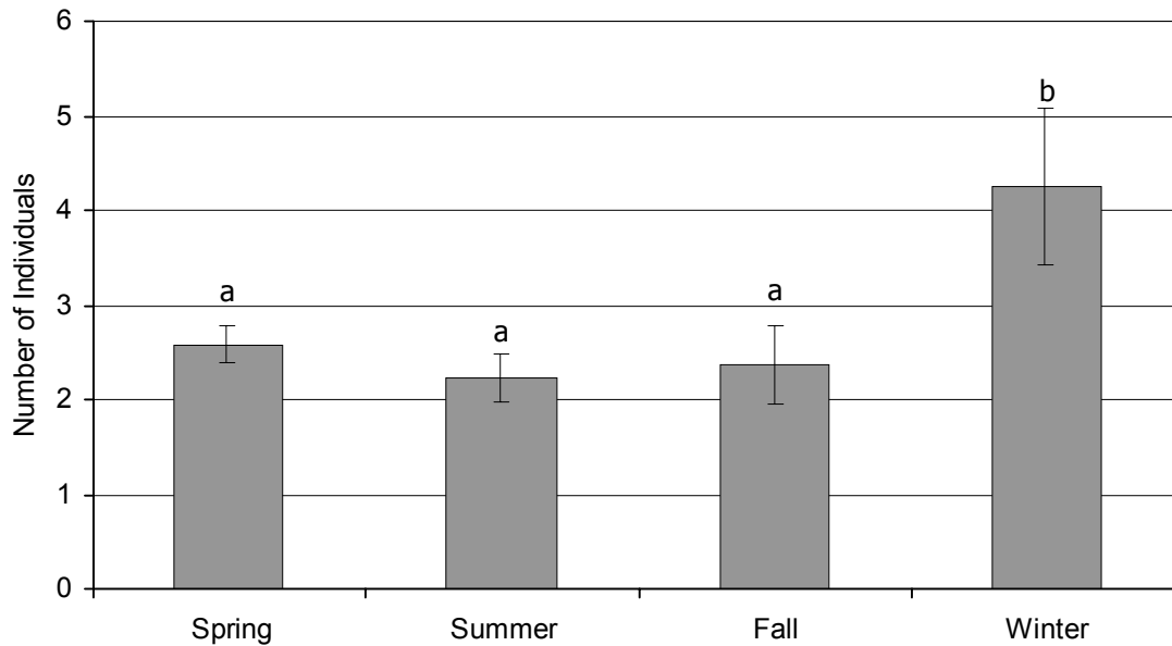
Figure 13. Mean group size of Dall's porpoise within the truncated distance, observed during Strait of Georgia surveys from May 1, 2000 to April 30, 2001. Bars are standard error. Letters denotes a significant difference.
