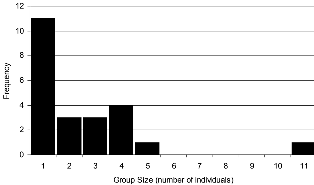
Figure 18. Frequency of harbour porpoise group size observed during surveys in the Strait of Georgia, May 1, 2000 to April 30, 2001.
