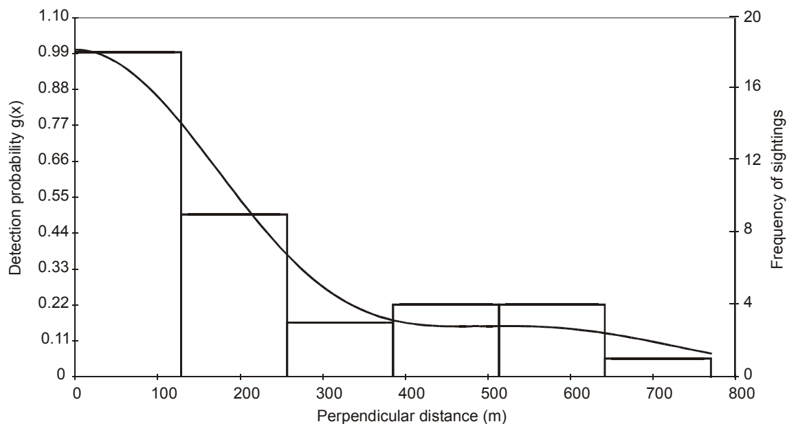
Figure 33. Probability detection distribution for perpendicular sighting distances of Steller sea lions. Bars represent the frequency of sightings and the line represents the half-normal/cosine model of best fit, truncated at 770 m.
