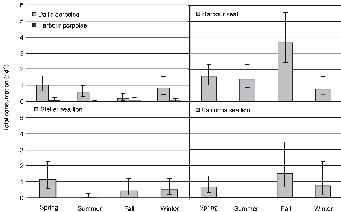
Figure 45. Comparison of estimated prey consumed by season ( t \cdot d^{-1} ) for marine mammal populations in the Strait of Georgia study area, modeled from abundance estimates. Ranges are calculated based on the 95% confidence intervals obtained from DISTANCE abundance estimates.
